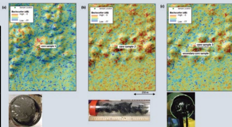
Figure 2: Backscatter displays at the location of core samples and their description. Data courtesy of TGS, Houston. (a) Large area of "popcorn" texture; location targets largest single mound with highest backscatter anomaly. Core is generally soft greenish-gray clay with no forams present and moderate cohesion and water content. Tar sediments on the top section with faint H_2S odor. (b) Large area of "popcorn" texture with high backscatter; location targets a mound (145-meter diameter) with high backscatter anomaly. (c) Unusual elliptical area of very low backscatter rimmed by high backscatter. Recovered 22-centimeters of black tar. Hydrocarbons present; classified as oil seep from Upper Jurassic marine carbonate.
