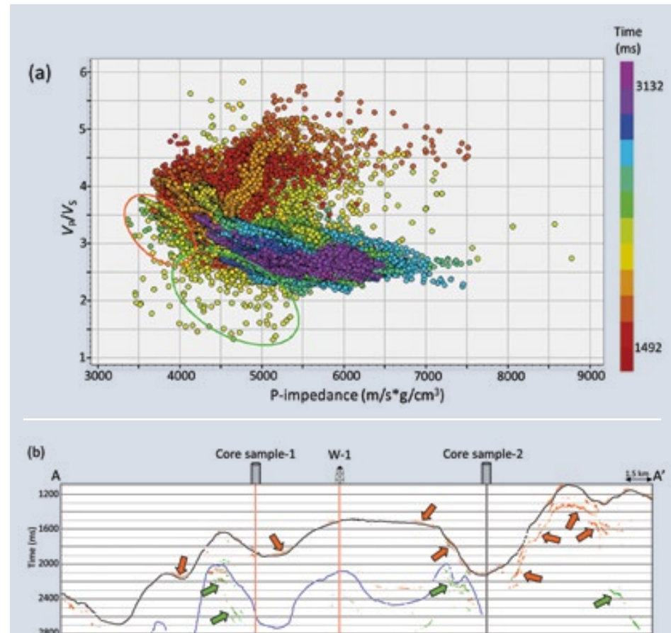
Figure 6: Crossplot of P-impedance versus V_p/V_s attributes. Cluster points with lower values of P-impedance and V_p/V_s could be associated with hydrocarbons; these cluster points are enclosed in the orange and green ellipses and back-projected on the vertical section AA' shown in (b). The block arrows indicate the location of prospective pockets. Data courtesy of TGS, Houston.
