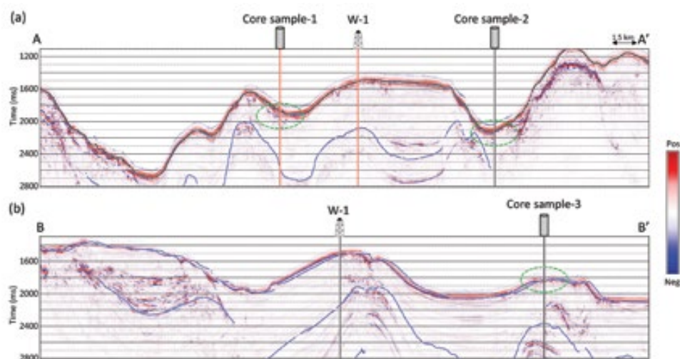
Figure 5: Fluid factor attribute along seismic lines AA' and BB' passing through well W-1. The location of the available core samples along the lines is shown. While core sample-1 falls on the line, core sample-2 is projected about 1.2 kilometers. Similarly, core sample 3 is projected 1.65 kilometers. Data courtesy of TGS, Houston.
